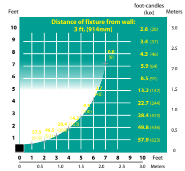
DL-04 Half Spread Photometric
