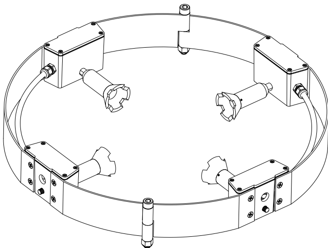
TRM-4 AUTOMATIC ADJUSTMENT
